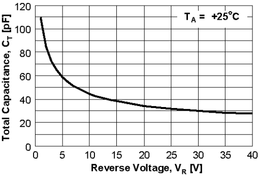
Total Capacitance
